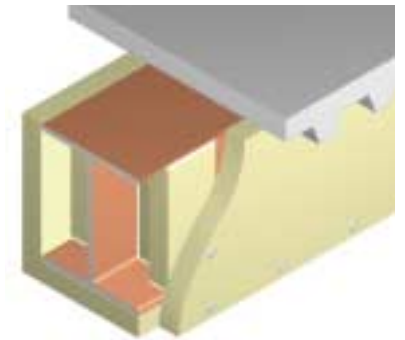
2 Alternative Tee-nogging arrangement (up to 2 hours fire protection)
